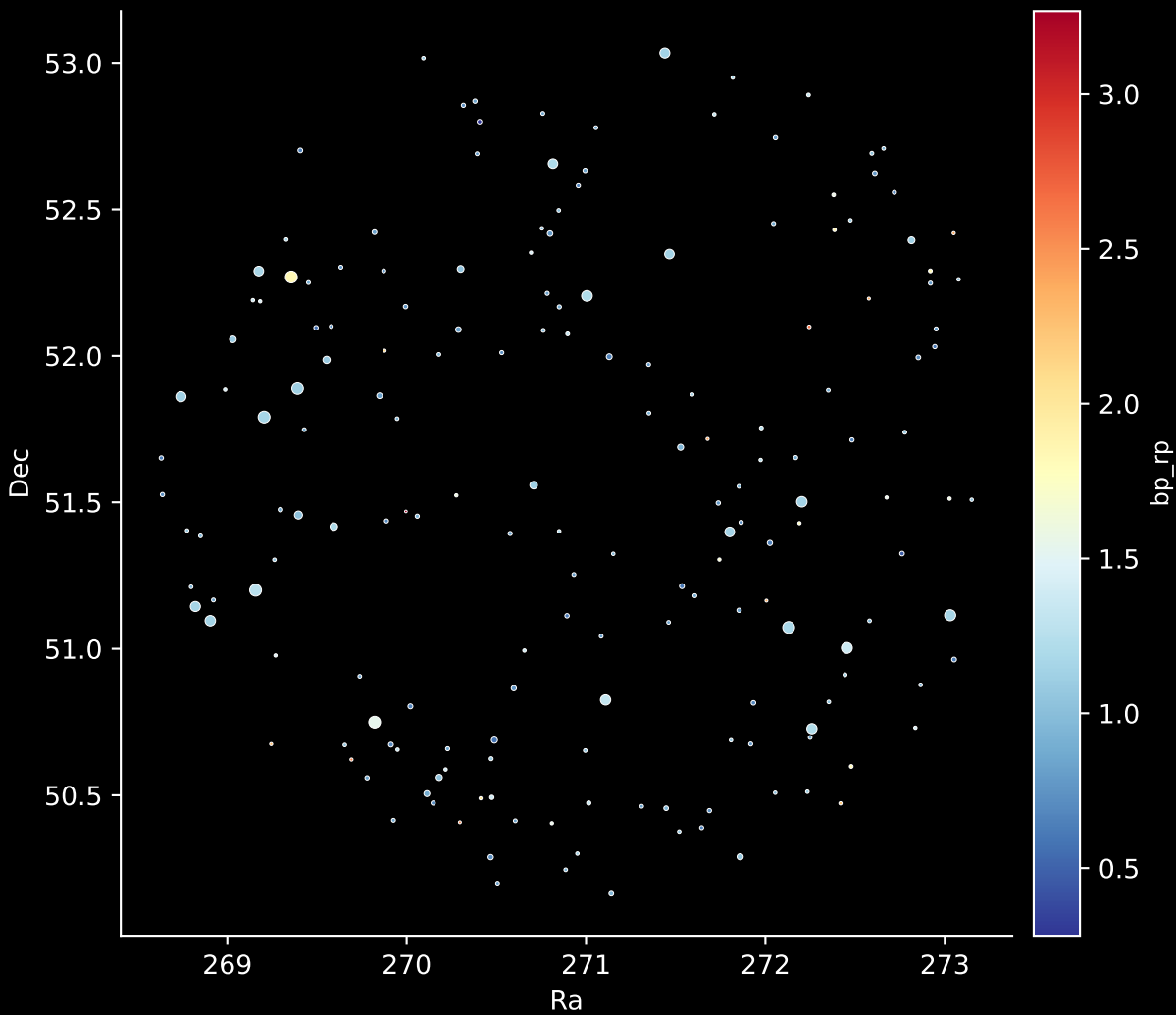
APOGEE DR17 Field: [151+60_MGA] Stars: 180
