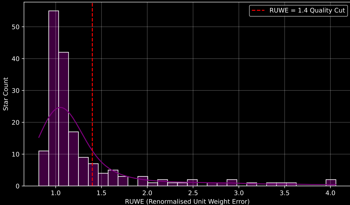
GAPOGEE DR17 Field [151+60_MGA] RUWE Distribution (n= 173)
