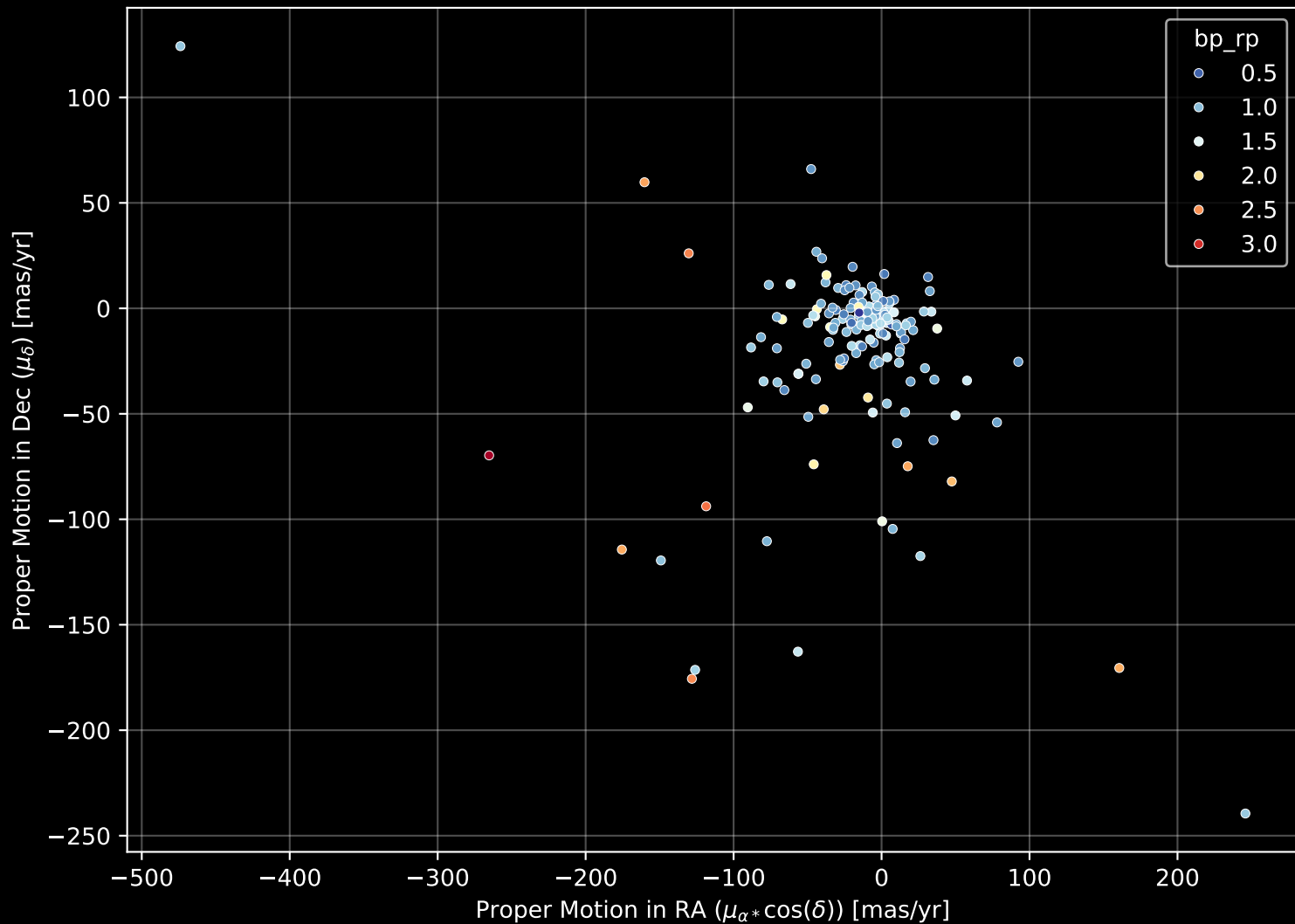
APOGEE DR17 Field: [151+60_MGA] Proper Motion Diagram (n= 180)
