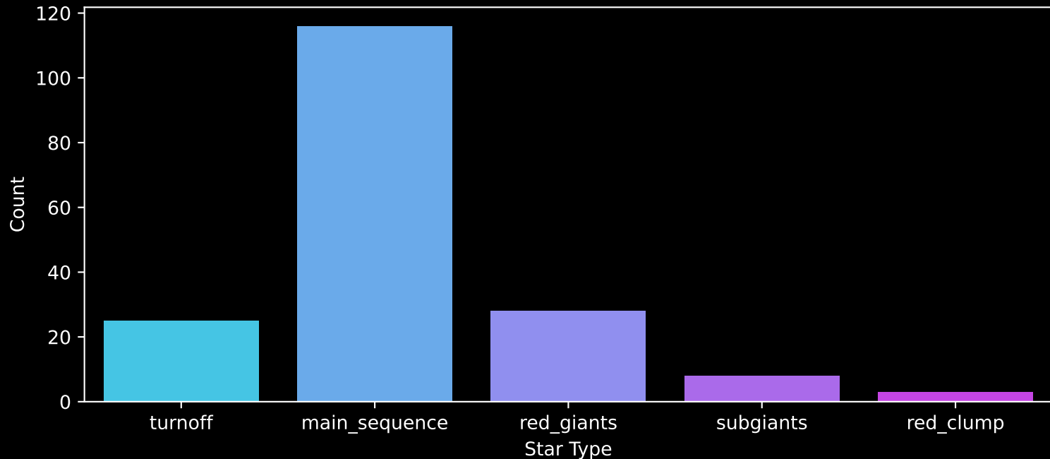
APOGEE DR17 Field: [151+60_MGA] Count plot of Star Type
