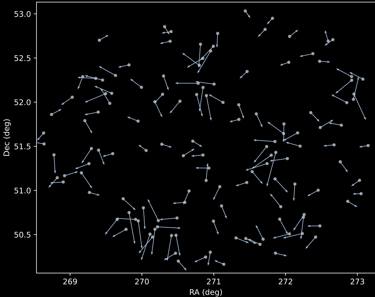
APOGEE DR17 Cluster 1 Proper Motion Vectors (n=134)
