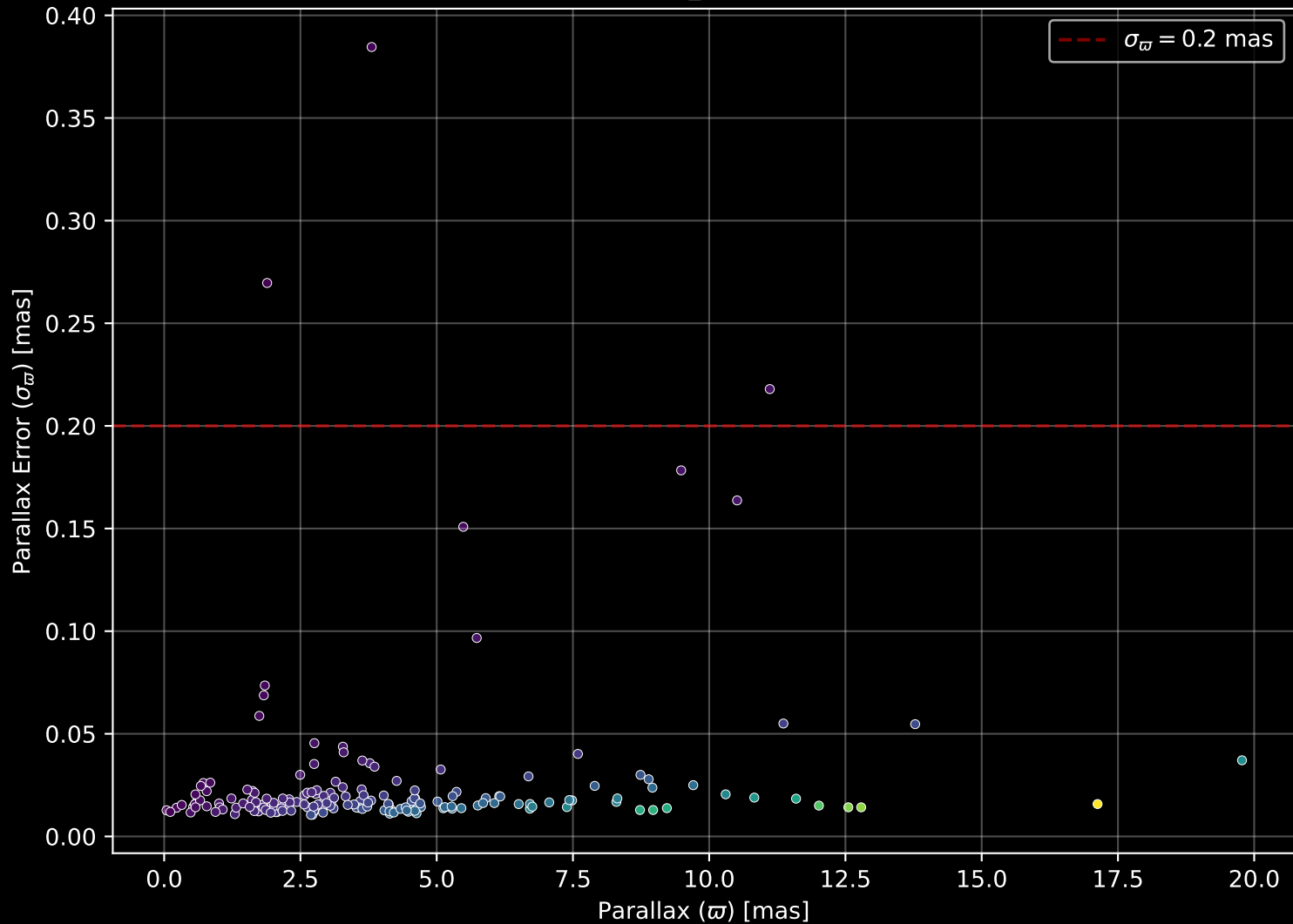
APOGEE DR17 Field: [151+60_MGA] Parallax Quality (n= 180)
